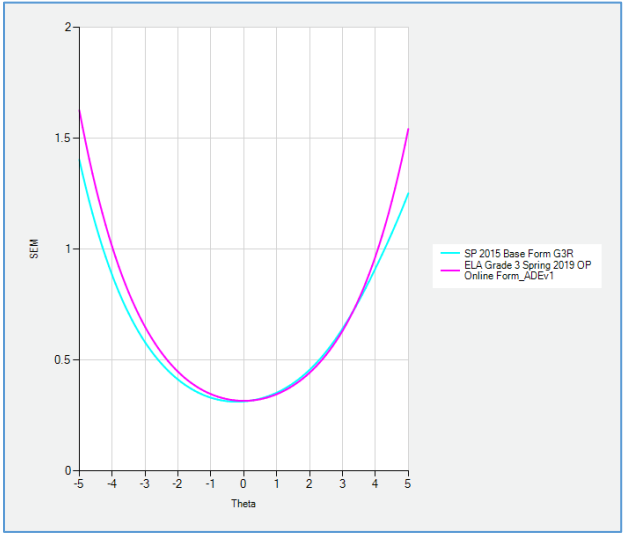
Standard Errors of Measurement
