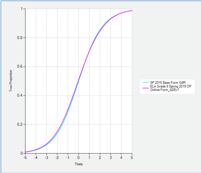
Test Characteristic Curves
