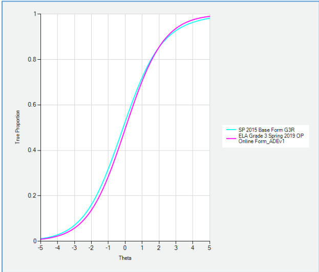
Test Characteristic Curves
